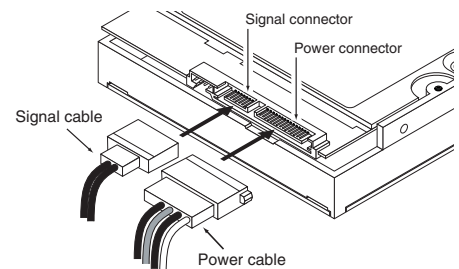
Figure 8. Attaching SATA cabling
