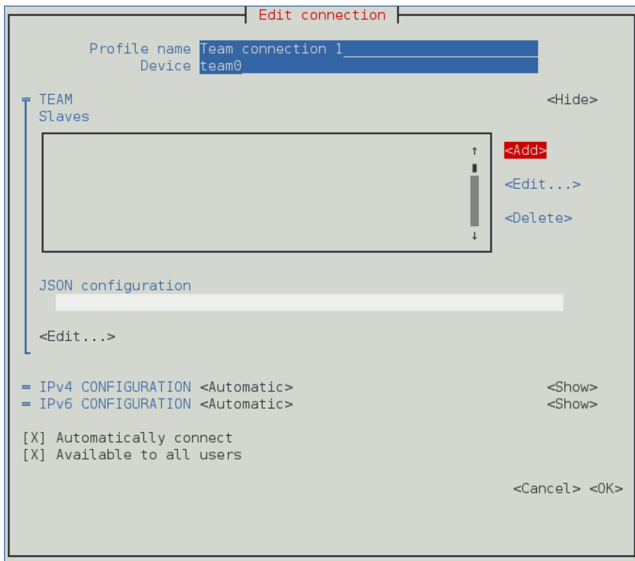
Figure 5.2. The NetworkManager Text User Interface Configuring a Team Connection menu
