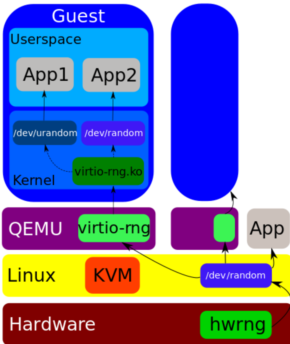
Figure 4.3. The virtio RNG device
