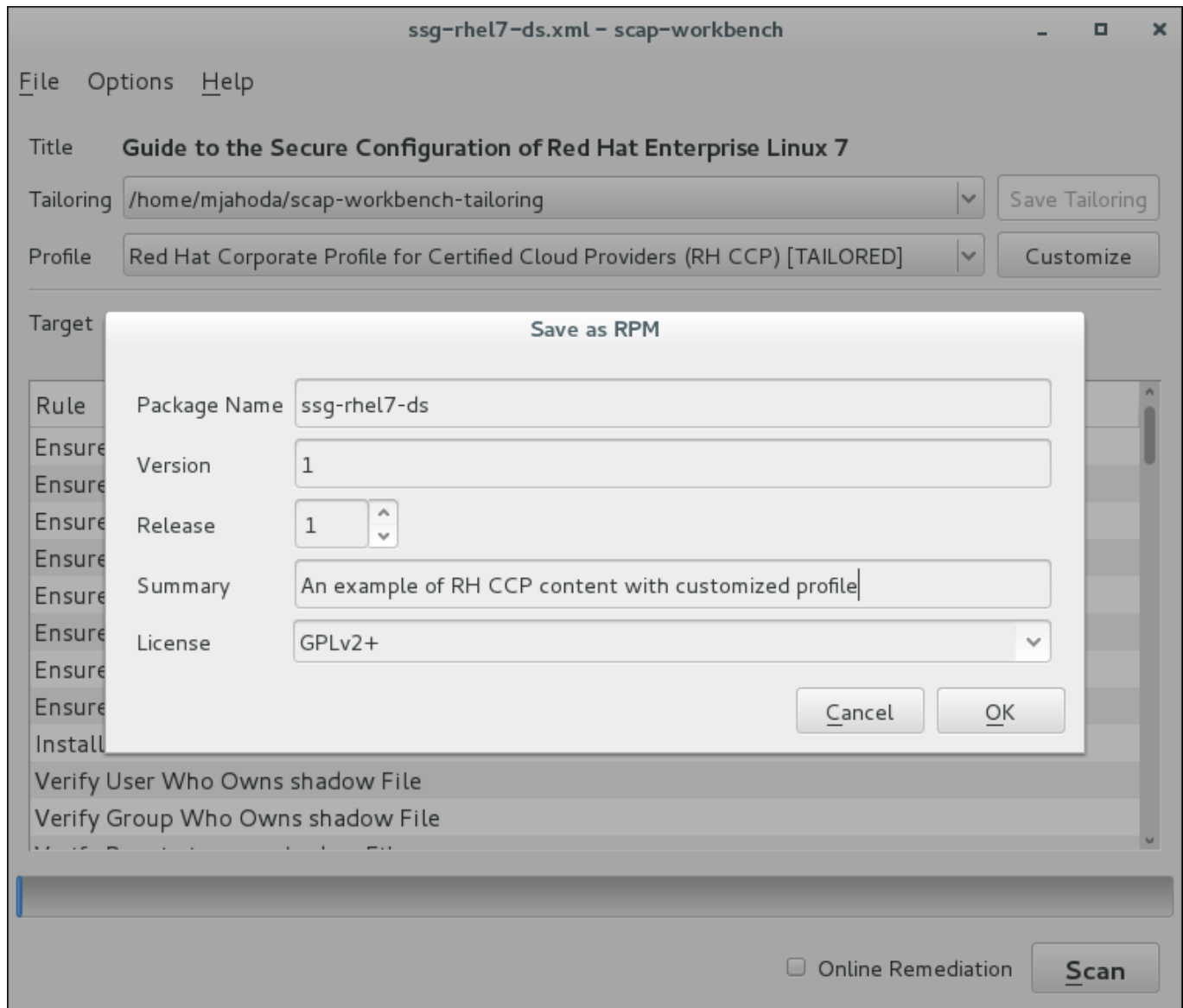
Figure 6.5. Saving the Current SCAP Content as an RPM Package
