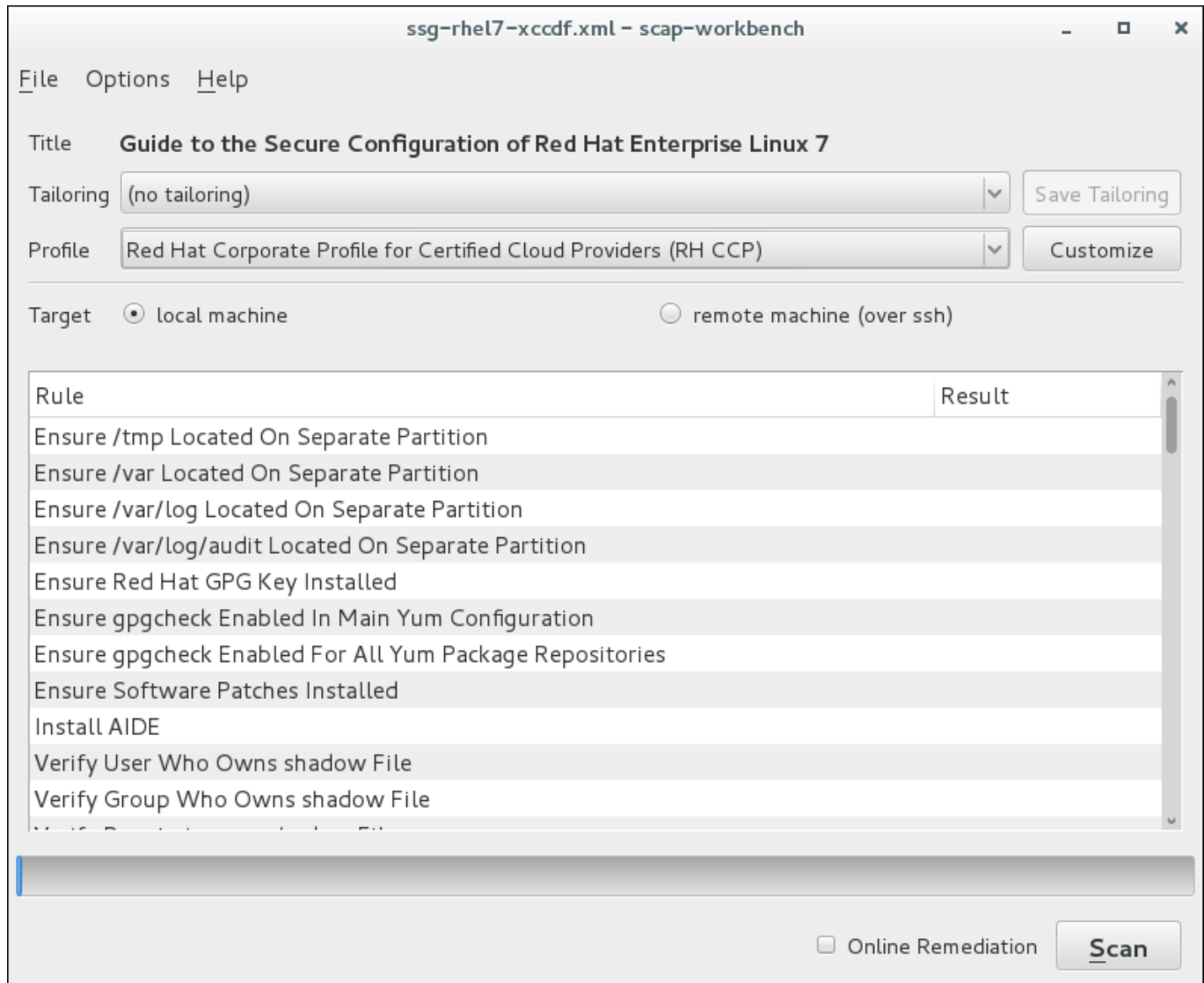
Figure 6.1. SCAP Workbench Window
